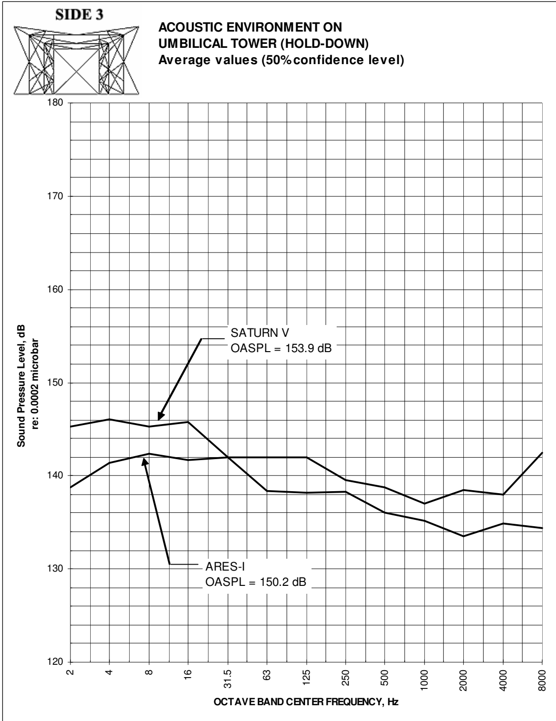
Figure 9: Zone 3.0 CLV and Saturn V Acoustic Environments (Hold-down)
