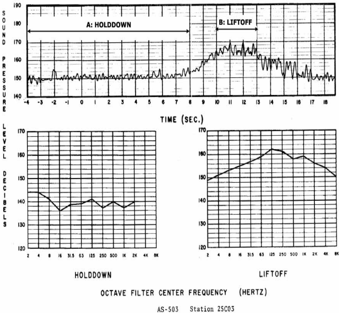
Figure 1. Acoustic Level on LUT
