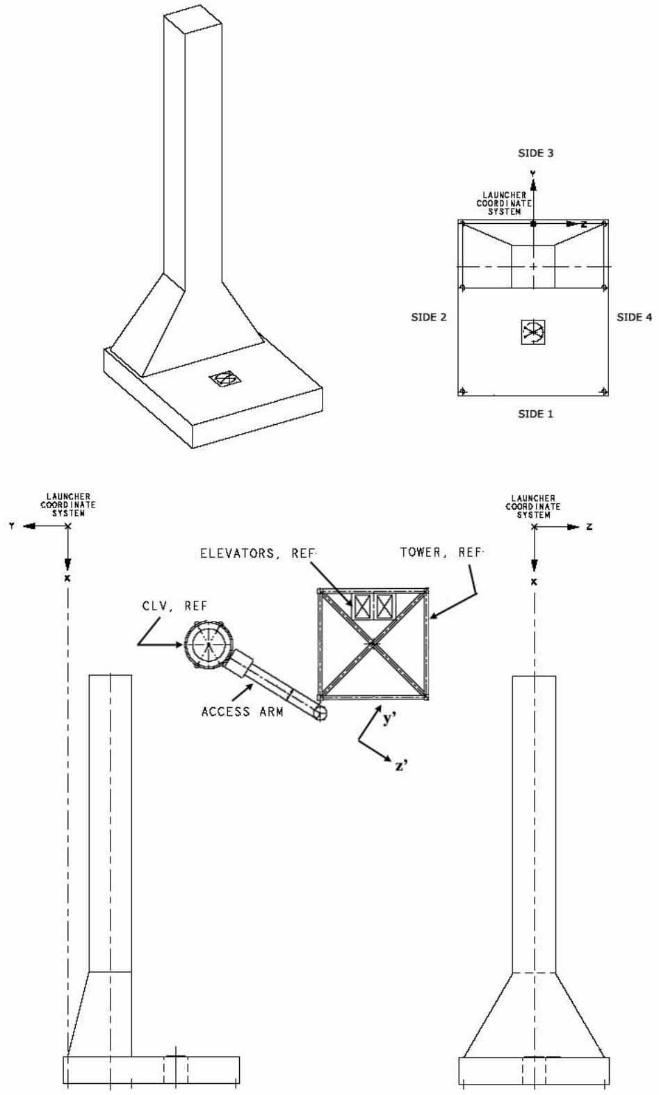
Figure 3: ML Base and Tower Coordinate System
