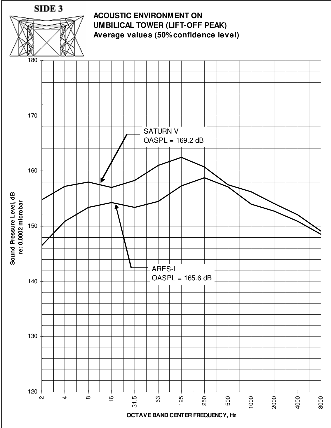
Figure 10: Zone 3.0 CLV and Saturn V Acoustic Environments (Lift-off)
