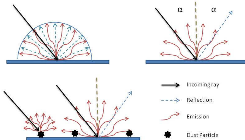
Figure 4: Types of Reflection
