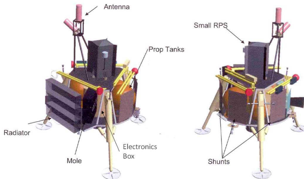
Figure 1: Nuclear Powered Lander
