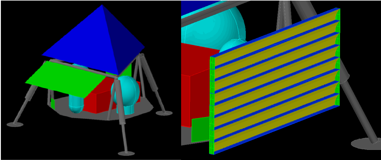
Figure 7: Radiators: Flat Plate Radiator (left) and Parabolic Radiator (right) - Fins (blue) with Parabolic Reflectors (yellow). For the recommended configuration the flat plate is placed above the solar arrays which requires a design change from what is shown.
