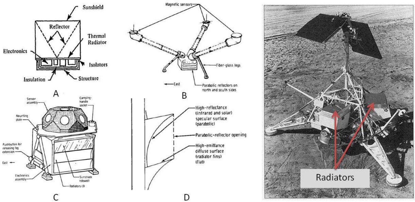
Figure 2: ALSEP (left) and Surveyor Spacecraft (right)
