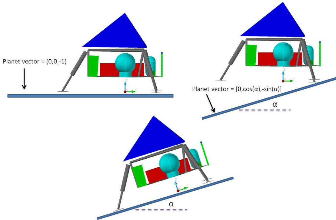
Figure 6: Surface Modeling using Thermal Desktop Orbit Command.
