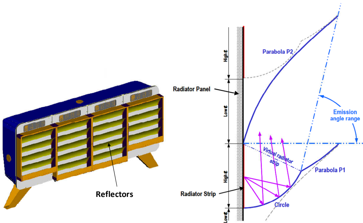
Figure 3: JWST Radiator: Baffled Assembly (left) and Reflector Side View (right) (5)
