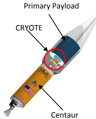
Figure 1: Proposed CRYOTE Launch Configuration – Atlas V EELV
