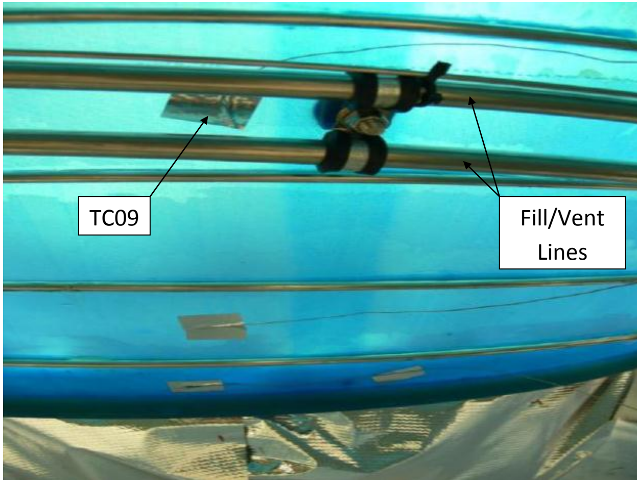
Figure 16: TC09 Location With Respect to Fill/Vent Lines
