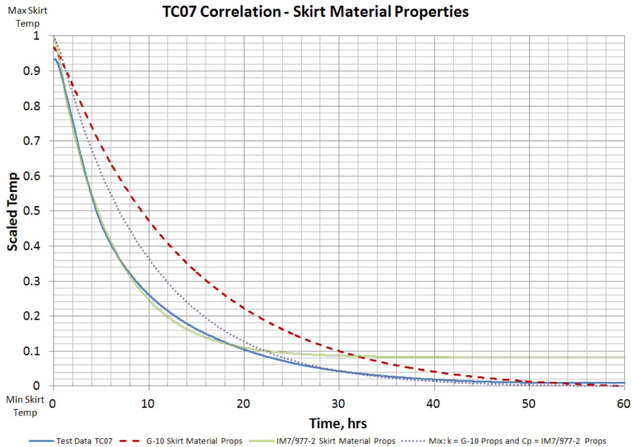
Figure 20: Analytical Trade Study: Skirt Material Properties
