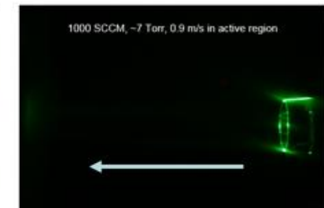
Precipitator on (~1400 volts, 500 \mu A)
