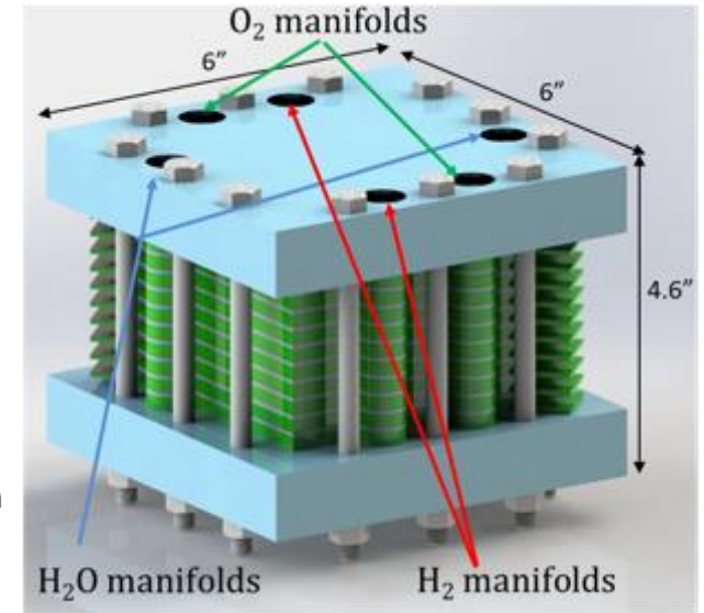
Electrolysis Cell Stack Design
