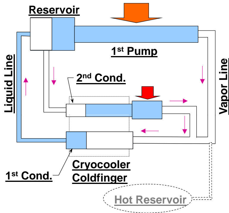
Normal Operation ( P_{SYSTEM} < 20\text{psia} )
